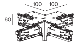
Internal power feeder*
