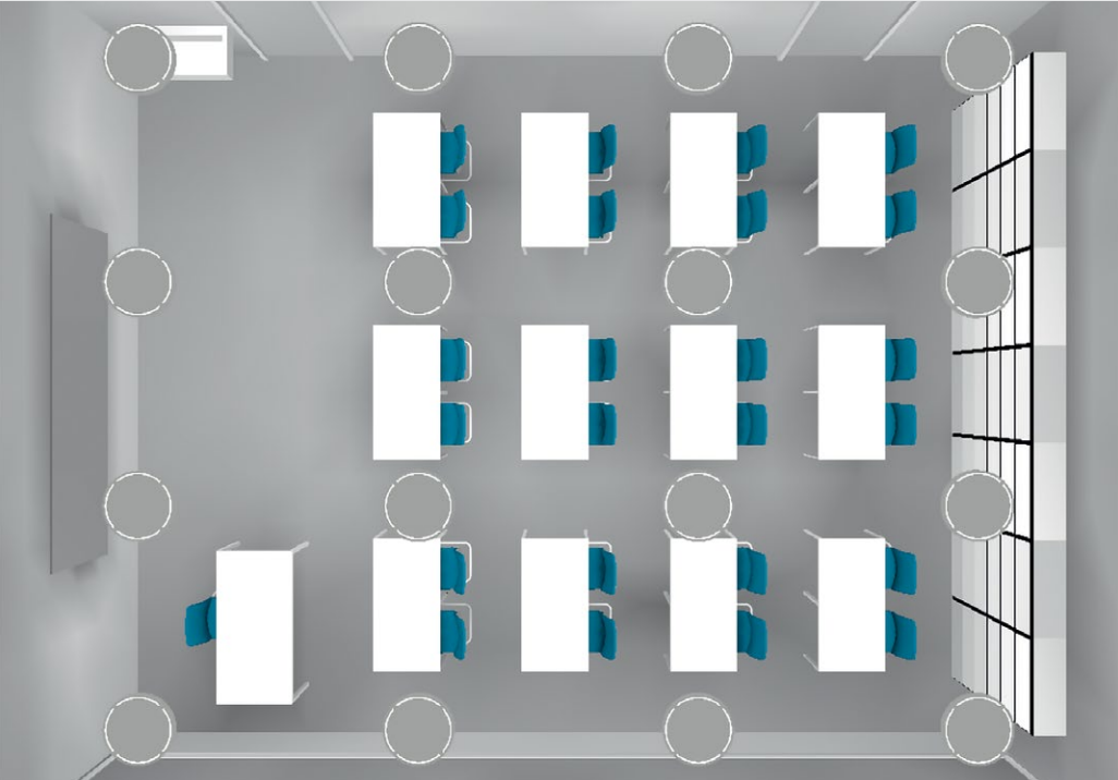
Room details Floor area: 9.35 × 7.5 m (70.1m²) Room height: 3m
